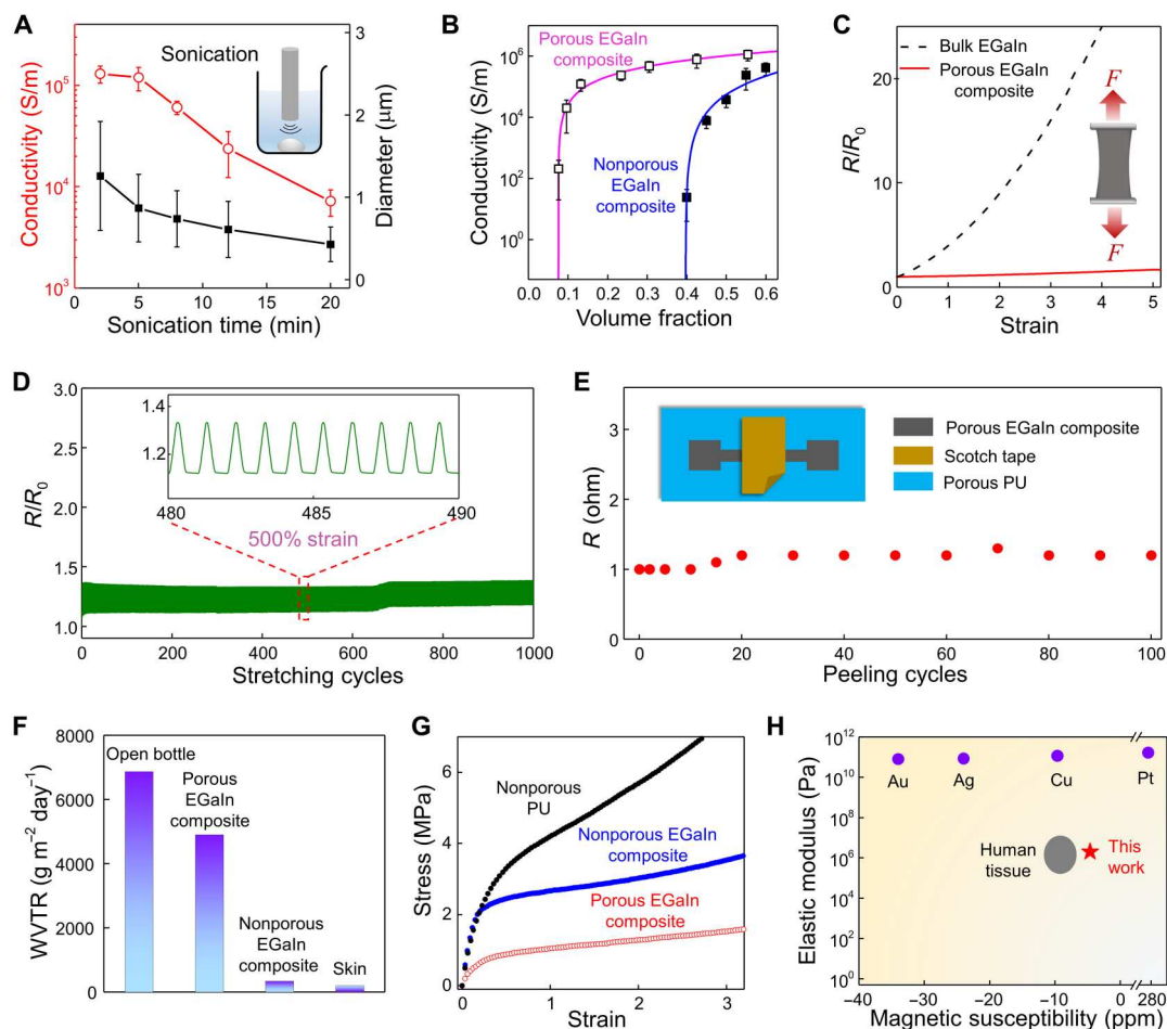
Fig. 2. Material characteristics and electromechanical responses. (A) EGaIn particle sizes (black) and electrical conductivities of porous EGaIn composites (red) as a function of the tip sonication time. Inset: Schematic illustration of tip sonication of bulk EGaIn in 1-butanol. (B) Electrical conductivities of nonporous and porous EGaIn composites as a function of EGaIn volume fractions. Error bars in (A) and (B) represent SDs of six samples. Pink and blue lines are fitting curves of porous and nonporous EGaIn composites, respectively, using the 3D percolation theory. (C) Relative resistance changes ( R/R_0 ) of bulk EGaIn and porous EGaIn composites as a function of uniaxial strains. (D) Relative resistance changes of porous EGaIn composites subjected to cyclic stretching (500% maximum strain). (E) Resistance changes of porous EGaIn composites under cyclic peeling with scotch tapes. The inset shows the testing setup. (F) Water vapor transmission rates (WVTRs) of an open bottle, porous EGaIn composites, nonporous EGaIn composites, and human skin. (G) Stress-strain curves of nonporous PU, nonporous EGaIn composites, and porous EGaIn composites, demonstrating the markedly reduced elastic modulus (i.e., ultrasoftness) of the porous EGaIn composite due to its porous structures. (H) Comparisons of the elastic modulus and magnetic susceptibility of porous EGaIn composites with some conventional metal conductors and human tissues. ppm, parts per million.
